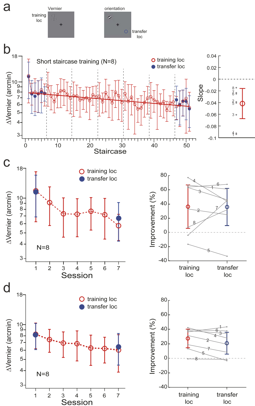
Figure 1. The training and transfer effects after double training with multiple short-staircase Vernier training and orientation training at the same location. (a) Stimulus configuration: The Vernier and the orientation tasks were trained at the same randomly selected retinal quadrant, and the transfer of Vernier learning was measured at a diagonal location (indicated by the blue circle, which was not shown in actual stimuli). (b) Left: The staircase-by-staircase changes of Vernier thresholds at the training (open symbols) and transfer (solid symbols) locations. The red line is the loglinear fit of the Vernier thresholds at the training location. Right: Individual (gray dot, each number representing a different observer) and mean (open circle) slopes of loglinear fits of the Vernier learning functions with short-staircase training. (c) Left: The session-by-session Vernier threshold changes at the training (open symbols) and transfer (solid symbols) locations when the first-staircase thresholds were used to represent session thresholds. Right: Individual (gray dot) and mean (open circle) percentage improvements at training and transfer locations. Each pair of gray dots connected by a gray line indicate a different observer’s data. (d) Left: The session-by-session Vernier threshold changes at the training (open symbols) and transfer (solid symbols) locations when the geometric means of all staircases in the corresponding pretraining and posttraining sessions were used to represent session thresholds. Right: Individual (gray dot) and mean (open circle) percentage improvements at training and transfer locations. Each pair of gray dots connected by a gray line indicate a different observer’s data. The error bars represent 95% CIs.
