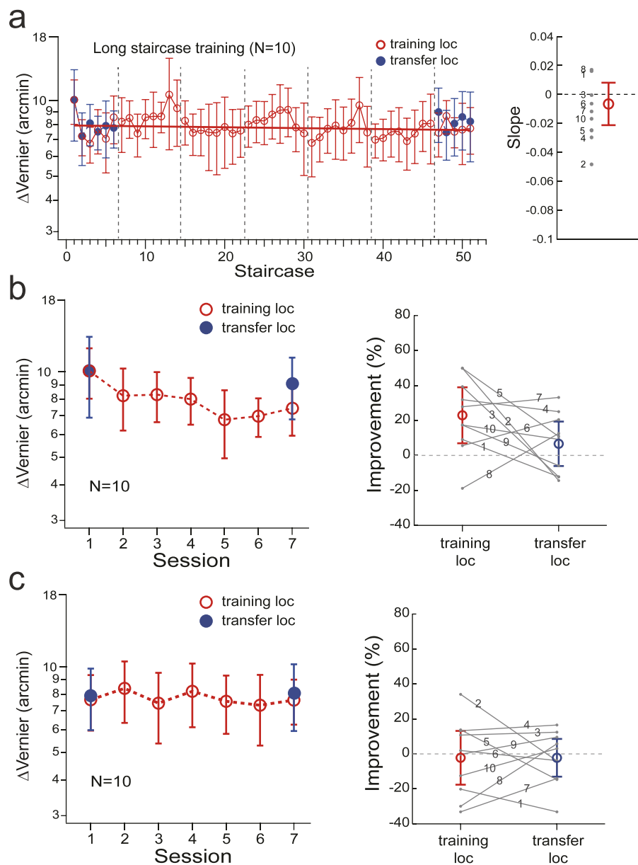
Figure 2. The training and transfer effects after double training with long-staircase Vernier training and multiple short-staircase orientation training at the same location. (a) Left: The staircase-by-staircase changes of Vernier thresholds at the training (open symbols) and transfer (solid symbols) locations. The red line is the loglinear fit of the Vernier thresholds at the training location. Right: Individual (gray dot) and mean (open circle) slopes of loglinear fits of the Vernier learning functions with long-staircase training. (b) Left: The session-by-session Vernier threshold changes at the training (open symbols) and transfer (solid symbols) locations when the first-staircase thresholds were used to represent session thresholds. Right: Individual (gray dot) and mean (open circle) percentage improvements at training and transfer locations. Each pair of gray dots connected by a gray line indicate a different observer’s data. (c) Left: The session-by-session Vernier threshold changes at the training (open symbols) and transfer (solid symbols) locations when the geometric means of all staircases in the corresponding pretraining and posttraining sessions were used to represent session thresholds. Right: Individual (gray dot) and mean (open circle) percentage improvements at training and transfer locations. Each pair of gray dots connected by a gray line indicate a different observer’s data. The error bars represent 95% CIs.
